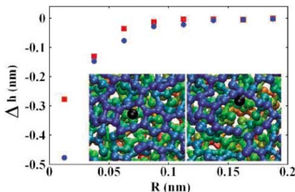
Fig. 1. Impact-induced height variation, \Delta h , as a function of the distance r from the impact point. The impacts of 1000 carbon atoms are simulated with classical MD for two impact energies: 30 eV (red squares) and 100 eV (blue dots). The average shape of \Delta h(r) indicates a trend toward crater formation. (Insets) Quantum MD of a single 100-eV carbon atom (black sphere) impinging with initial velocity perpendicular to the plane. (Left) Snapshot of the initial configuration. (Right) Formation of a small crater after 1 ps. The substrate atoms are color coded according to their initial position in the film. The relative movement of the black sphere in the right inset with respect to the left inset is a consequence of multiple collisions following impact.
